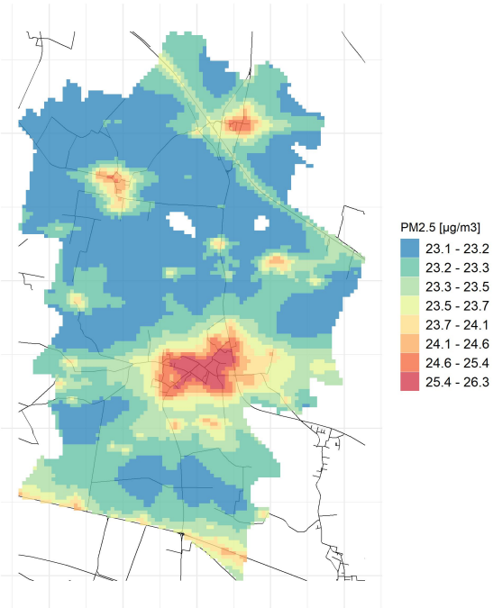
Conc. media annua PM2.5
