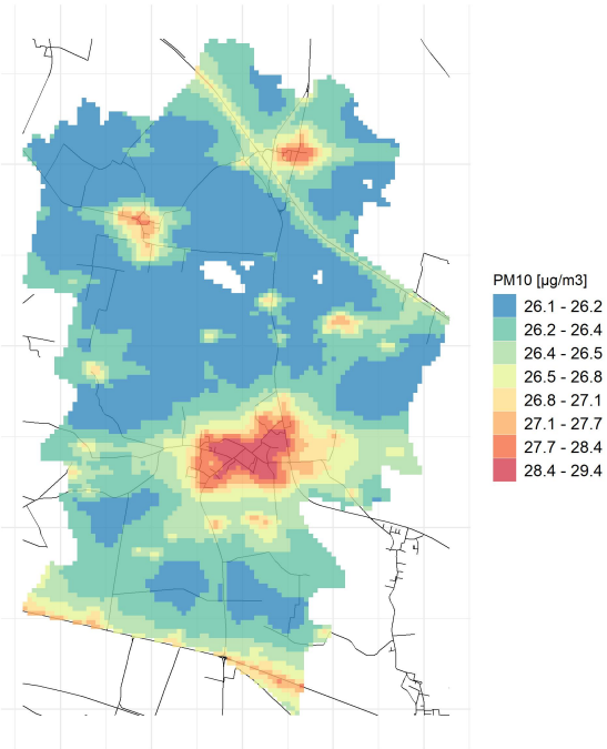
Conc. media annua PM10
